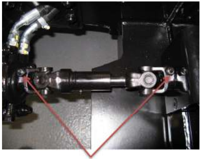
Steering box to bevel box inter shaft U/J pinch bolts
